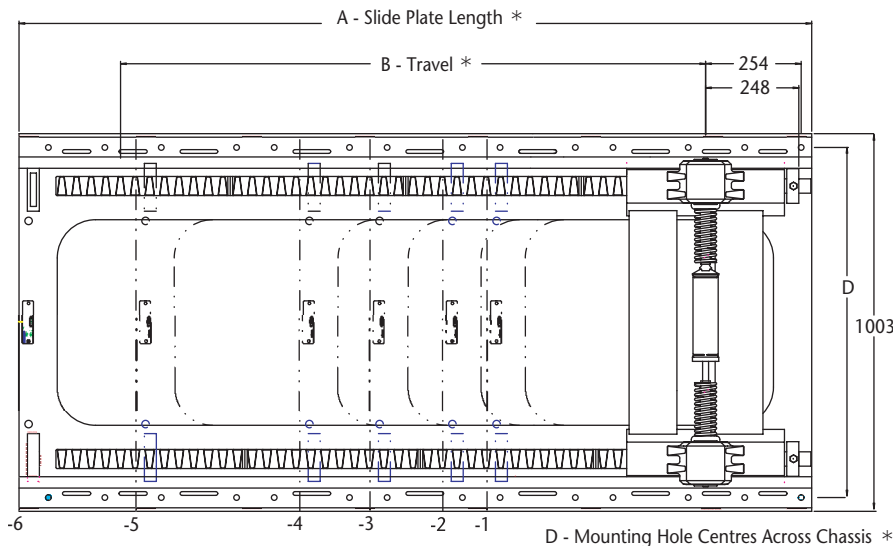
196mm and 221mm high assembly
