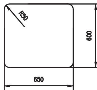
Material: Stahl/Steel
