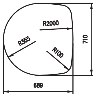
Material: Aluminium Querschnitt/Cross section: F05
