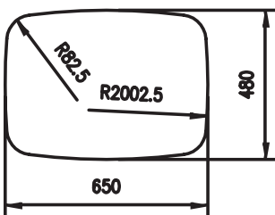
Material: Aluminium Querschnitt/Cross section: 921
