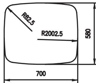
Material: Aluminium Querschnitt/Cross section: 923
