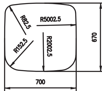
Material: Aluminium | Stahl/Steel Querschnitt/Cross section: F07
