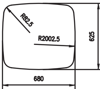
Material: Aluminium Querschnitt/Cross section: 922
