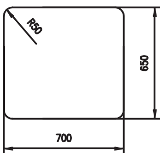
Material: Stahl/Steel
