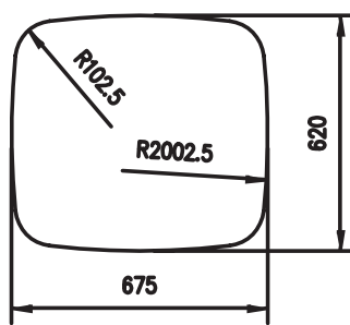
Material: Aluminium Querschnitt/Cross section: 872
