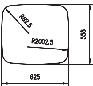
Material: Aluminium Querschnitt/Cross section: 824
